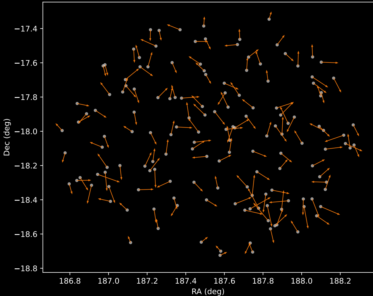
GALAH DR4 Cluster 2 Proper Motion Vectors (n=152)
