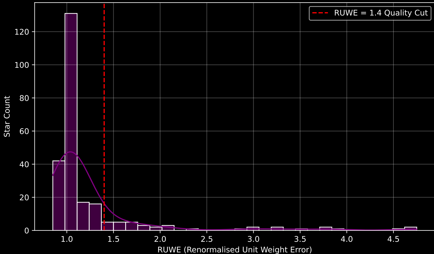
GALAH DR4 Field [1948] RUWE Distribution (n= 242)
